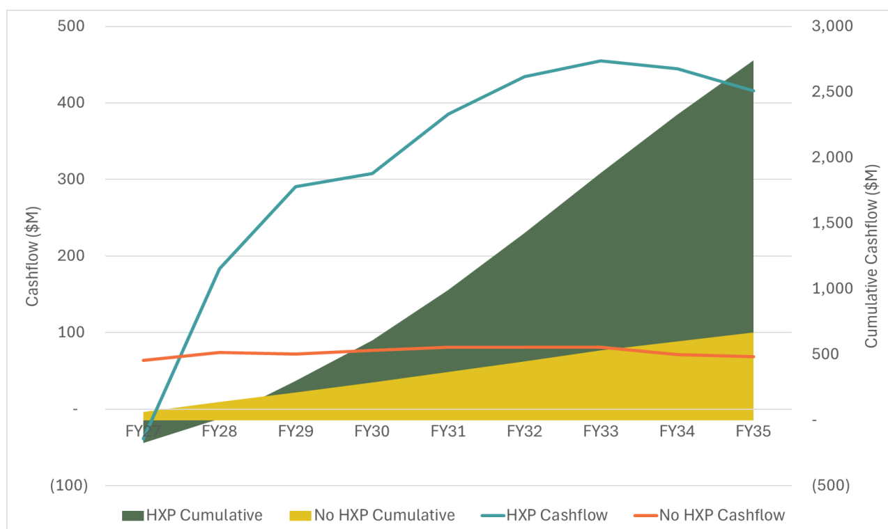
Figure 3 - HXP Cashflow (Gold Price - $4,905/oz)
